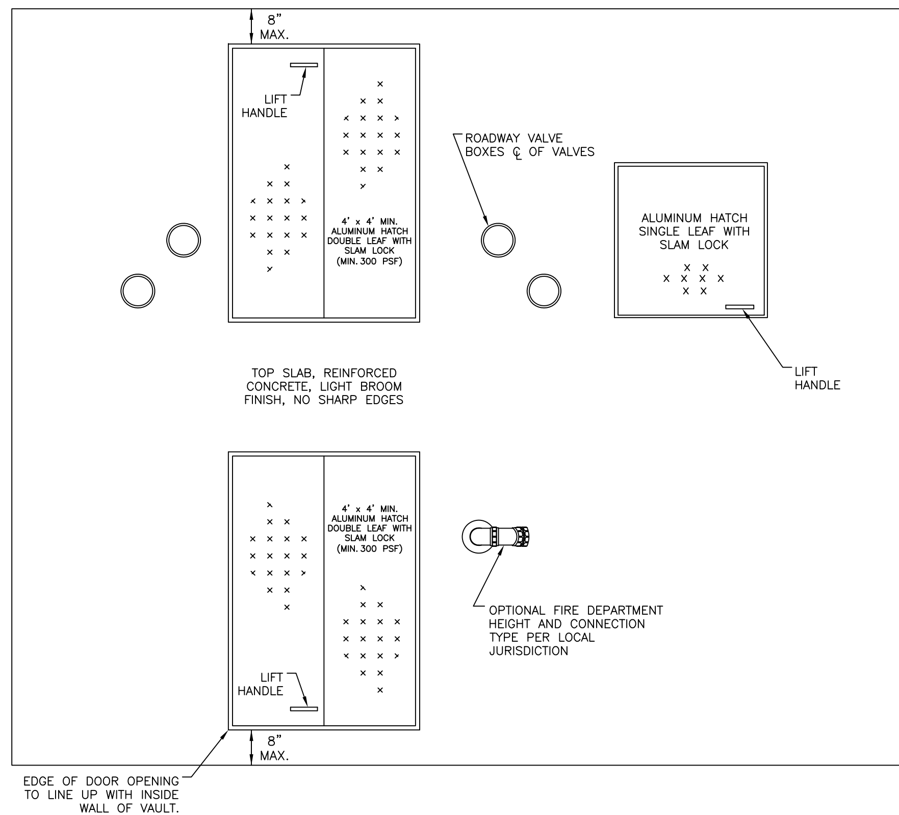
TOP SLAB NTS
