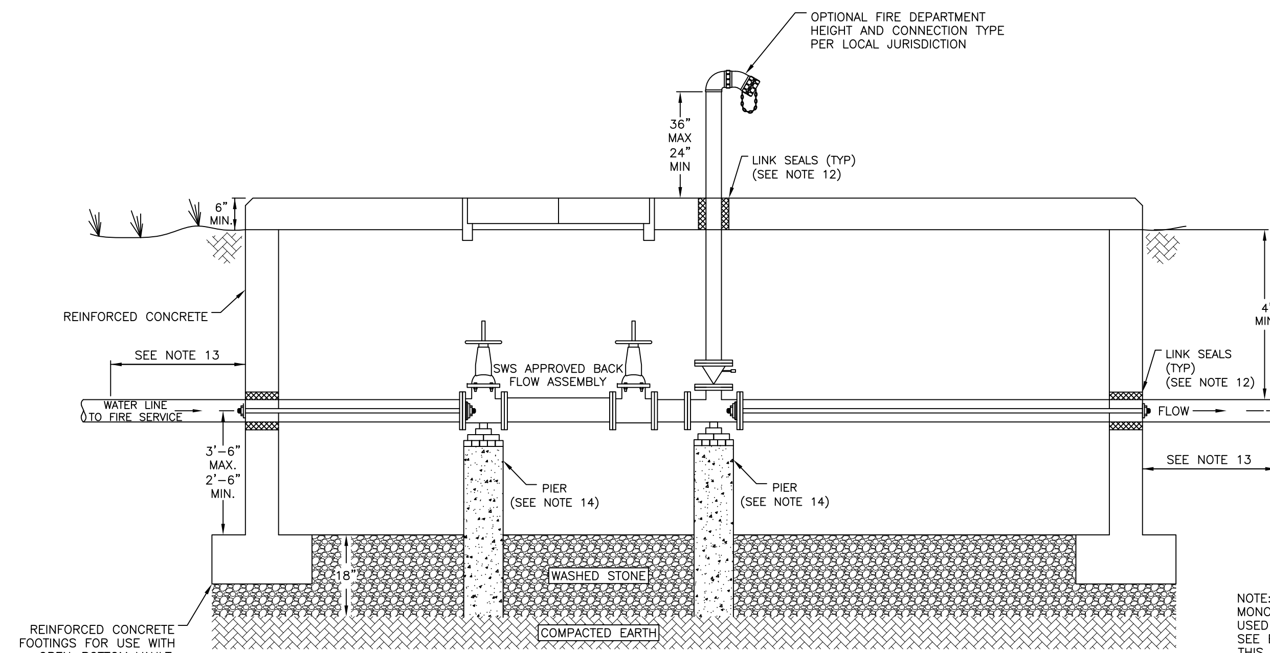
SECTION B-B NTS
